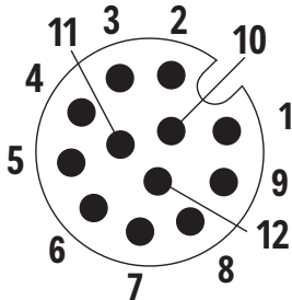
Schematic Diagram - M12, 12-pin, A-coded, male
